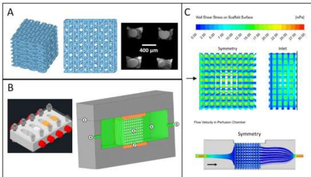
Figure. A: Left: Scaffold with 45° layer geometry. Right: Population of scaffold (90° geometry). Pores filled with cells one week after seeding (transmission image). B: Left: 3D model of the perfusion multi-biochamber (left). Right: Model of the free fluid space within chamber and scaffold created with Ansys (fluid space divided vertically at symmetry plane). C: Top: Wall shear stress at scaffold surface calculated in Ansys (color map). ‘Symmetry’ shows a cross-section in flow direction, ‘Inlet’ the scaffold surface at the inlet side. Bottom: Colored streamlines of flow velocity within the biochamber at the symmetry plane.
